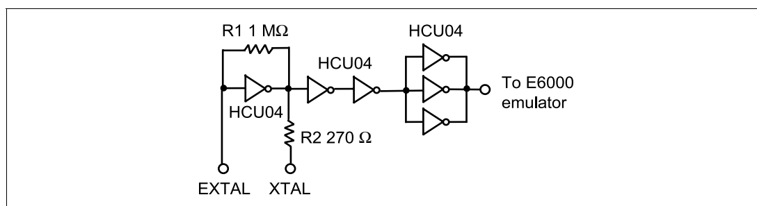
Figure 10 Clock Oscillator Circuits
